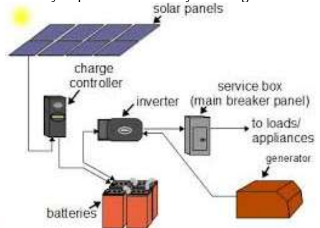
Figure 2. Production process from solar panels [5]. How does this happen?
