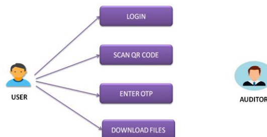
Figure 2: Mobile App
