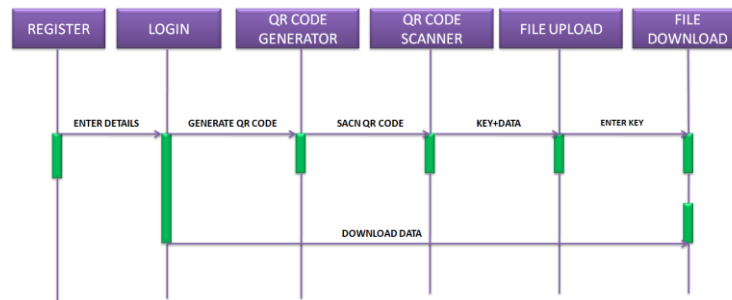
Figure 3: Sequence Diagram
