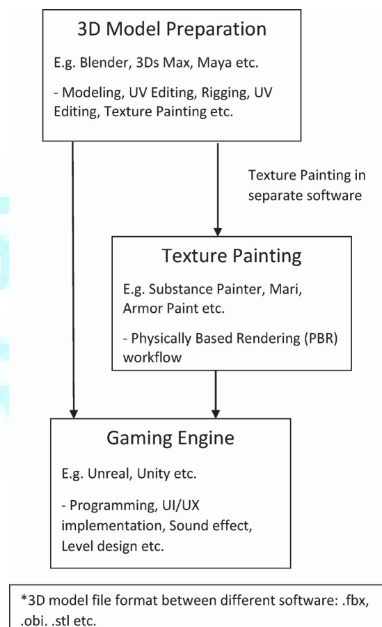
Figure 1. The flow chart of the VR program development. The development process includes modeling, texture mapping and VR programming.
