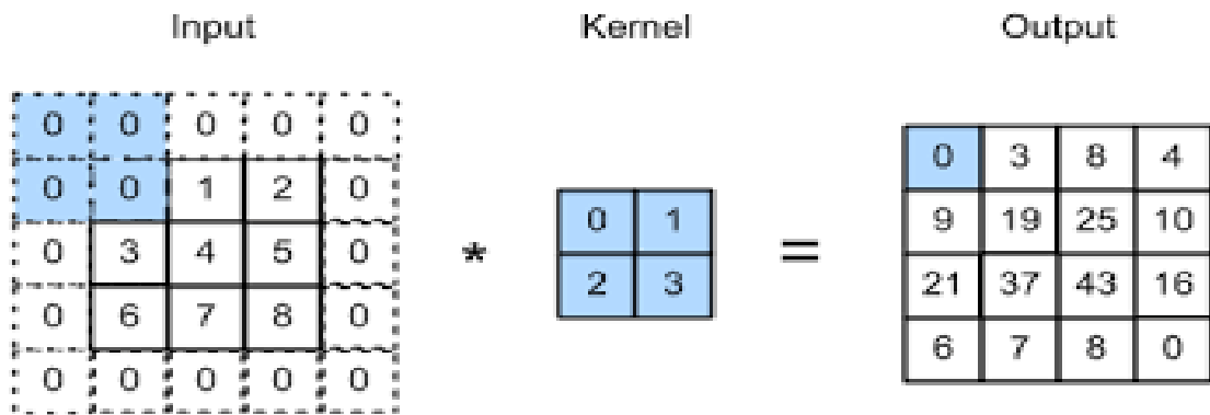
“Fig. 4. Padding is applied to reduce the information loss from corners of image”
