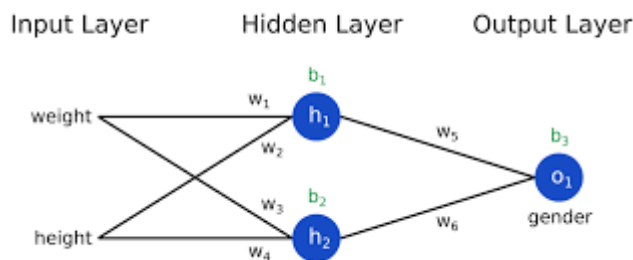
“Fig. 5. It shows a simple neural network having input neurons and hidden layers which are initially given weights and inputs to calculate desired output using optimisation algorithms.”
