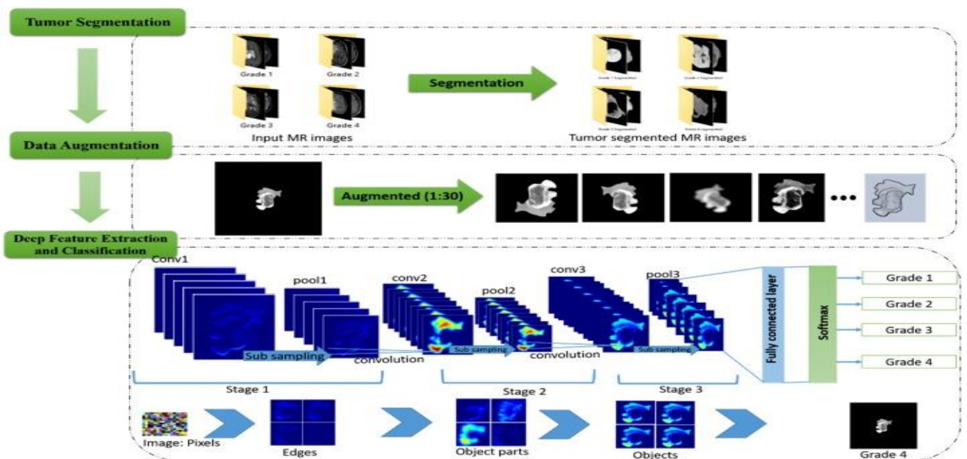
“Fig.6 Network architecture of CNN having different layers (A) convolutional layer to reduce size of image (B) pooling layer to retain maximum intensity in images (C) fully connected layer to give 1D input to each neuron and apply softmax function to classify output.”
