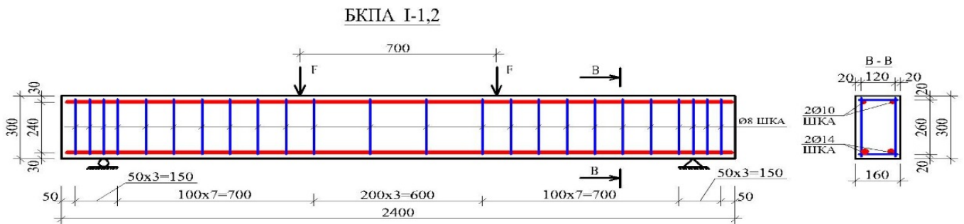
Figure 1. Fitting and loading schemes of sample barriers.
