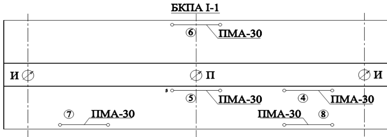
Figure 2. Location and installation schemes of measuring devices on sample barriers;
